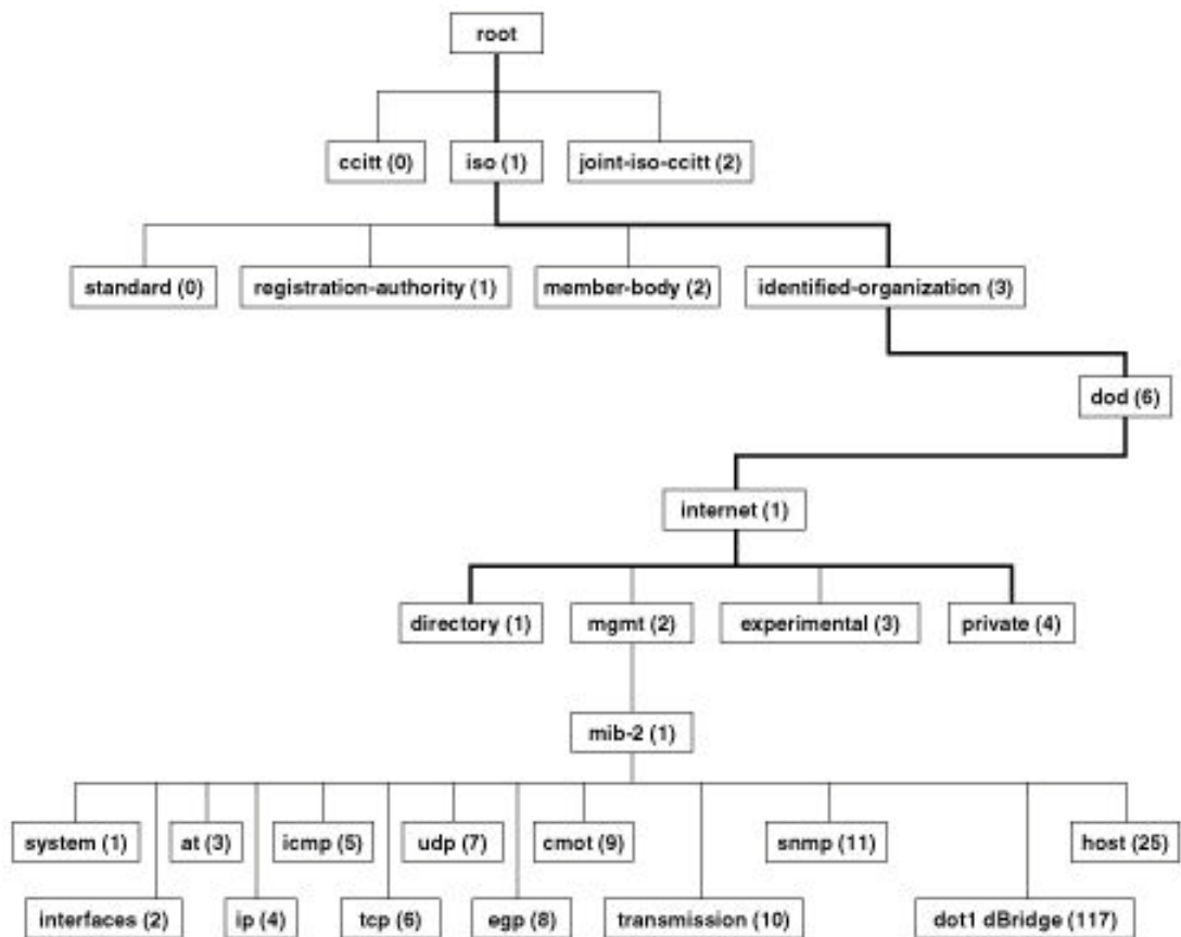
Figure 69. MIB Tree
